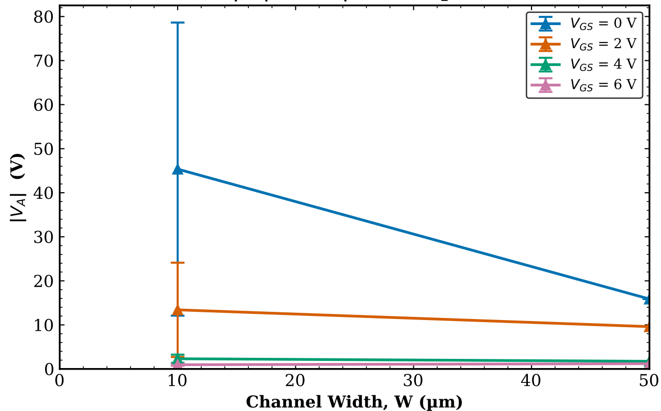
TFT2 Combined (Tr. 1 & 2) |V_A| vs W | L = 20\text{ }\mu\text{m}
